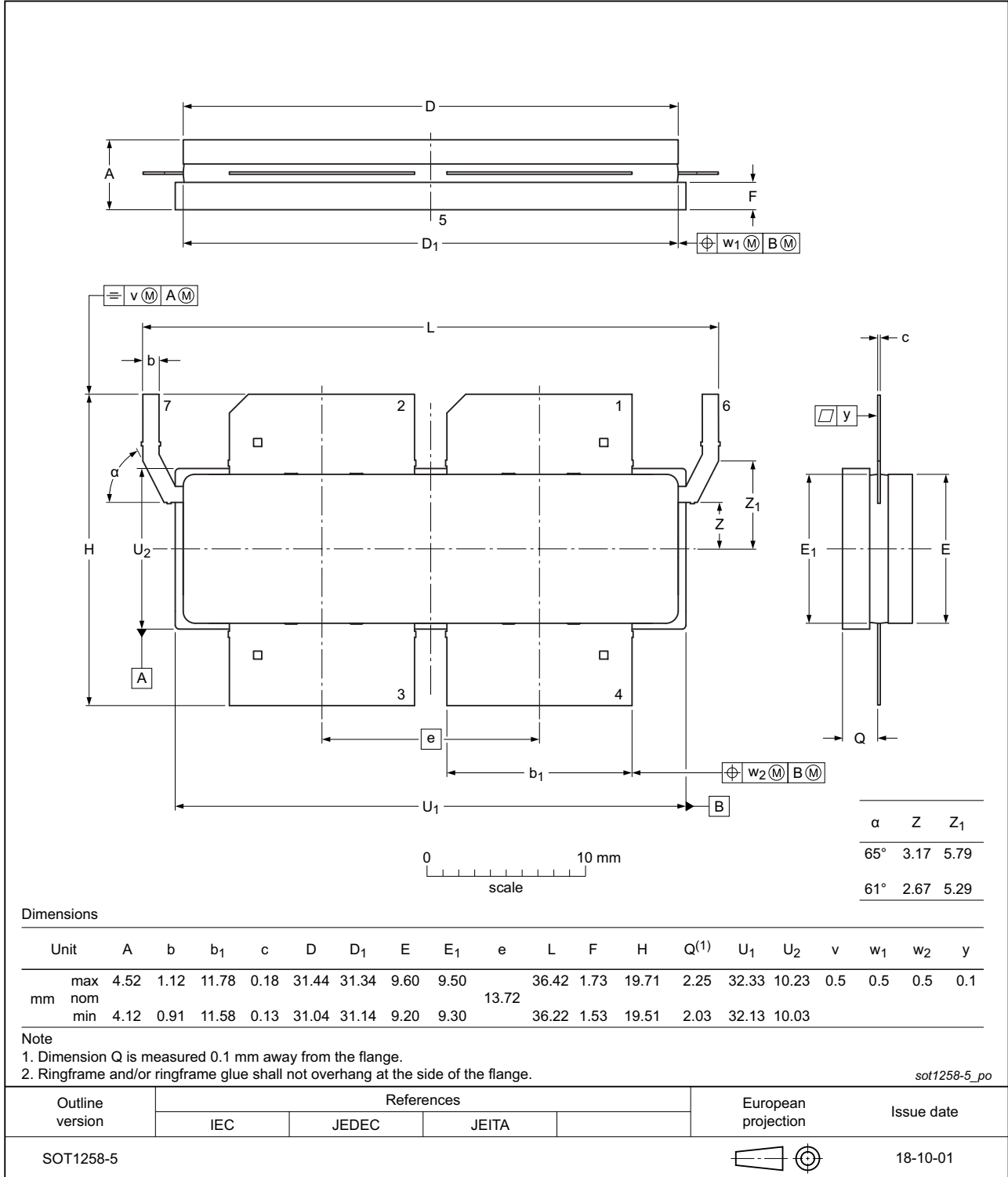
Fig 12. Package outline SOT1258-5
