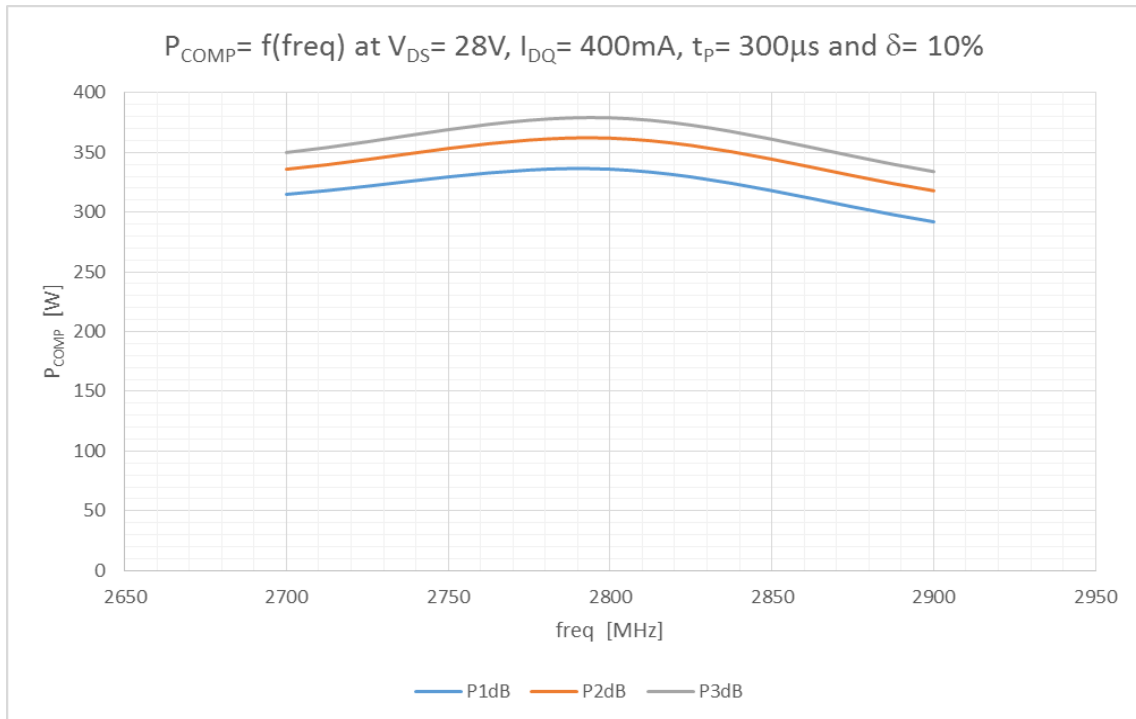
Figure 4 Compressed Power
